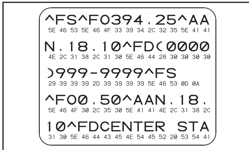
Figure 18. Communications Diagnostics Test Sample Printout
